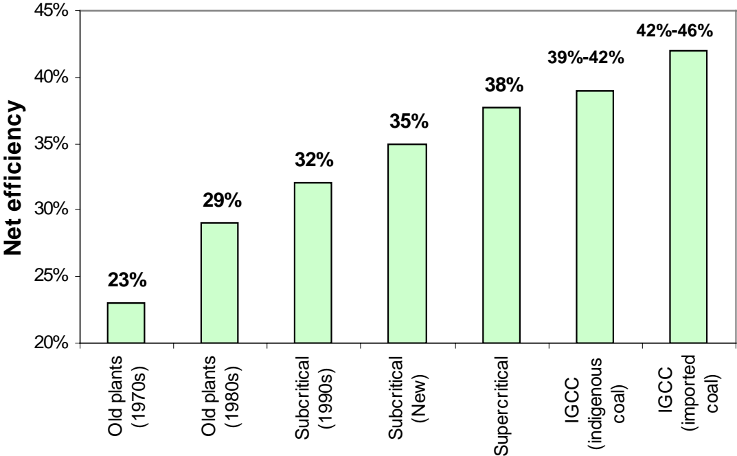
Figure 9 : Improvement in power plant efficiencies with up-gradation of technology
