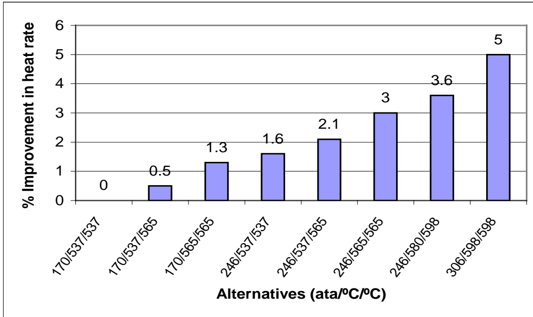
Figure B1 Improvement in Heat Rate with Steam Parameters
