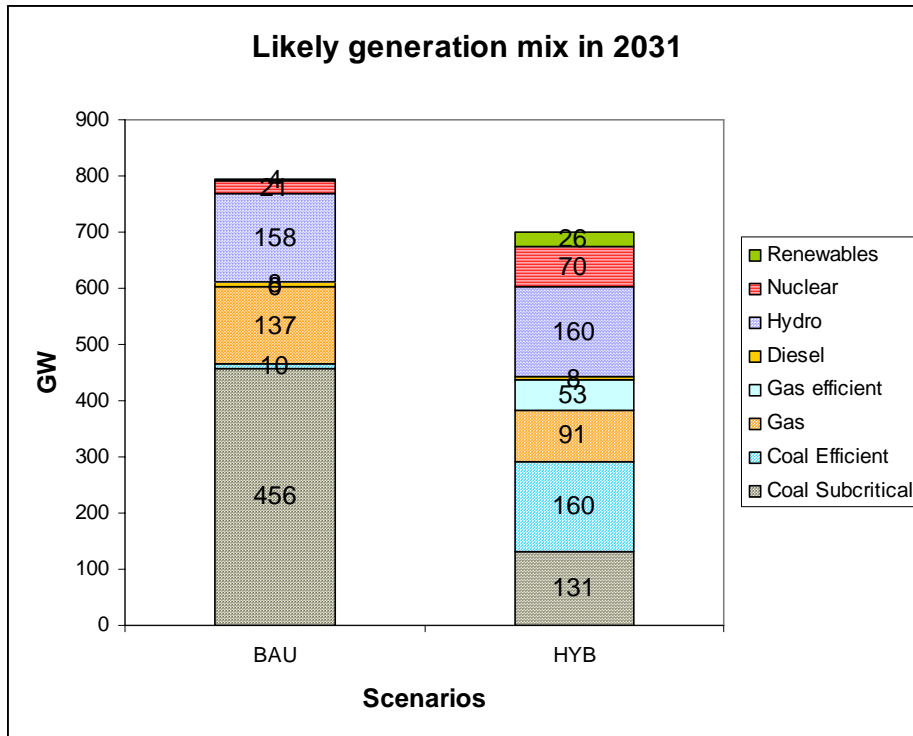
Figure 10 : Comparison of likely power generation mix in 2031
