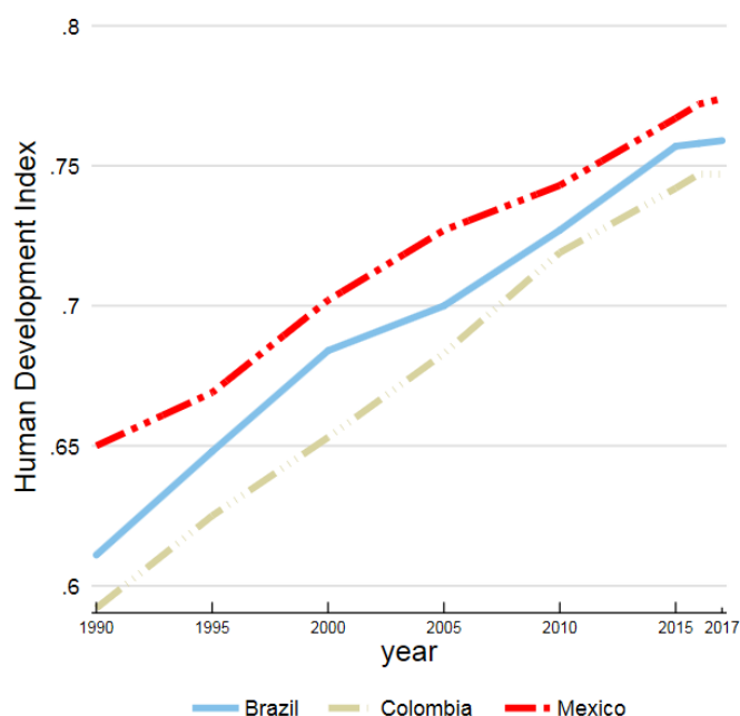
Figure 2: HDI trends for Brazil, Colombia and Mexico, 1990-2017
