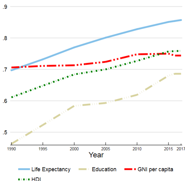
Figure 1: Trends in Brazil's HDI component indices 1990-2017
