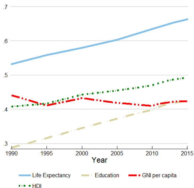
Figure 1: Trends in Haiti's HDI component indices 1990-2015
