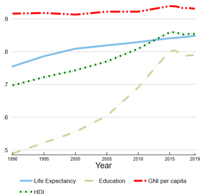
Figure 1: Trends in Saudi Arabia's HDI component indices 1990-2019
