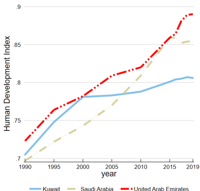
Figure 2: HDI trends for Saudi Arabia, Kuwait and United Arab Emirates, 1990-2019
