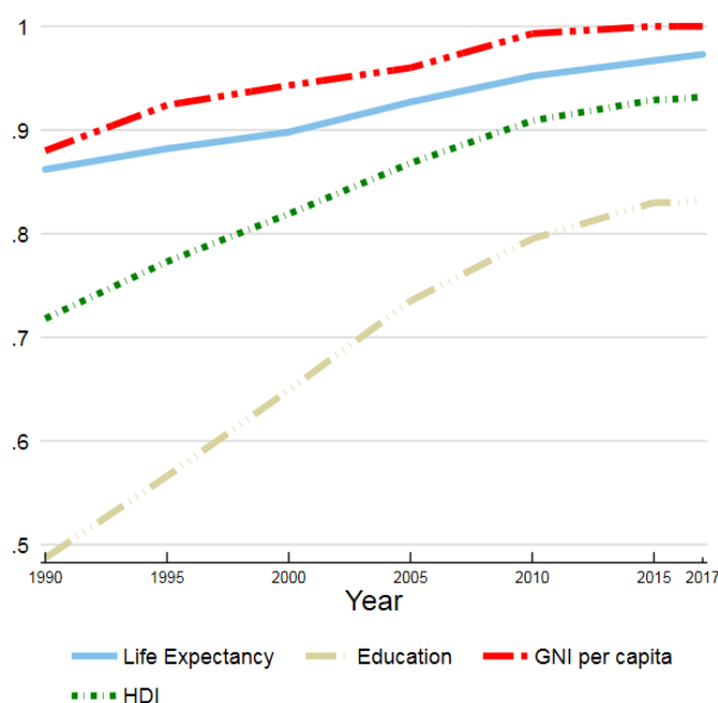
Figure 1: Trends in Singapore’s HDI component indices 1990-2017
