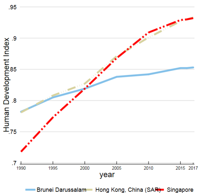
Figure 2: HDI trends for Singapore, Hong Kong, China (SAR) and Brunei Darussalam, 1990-2017
