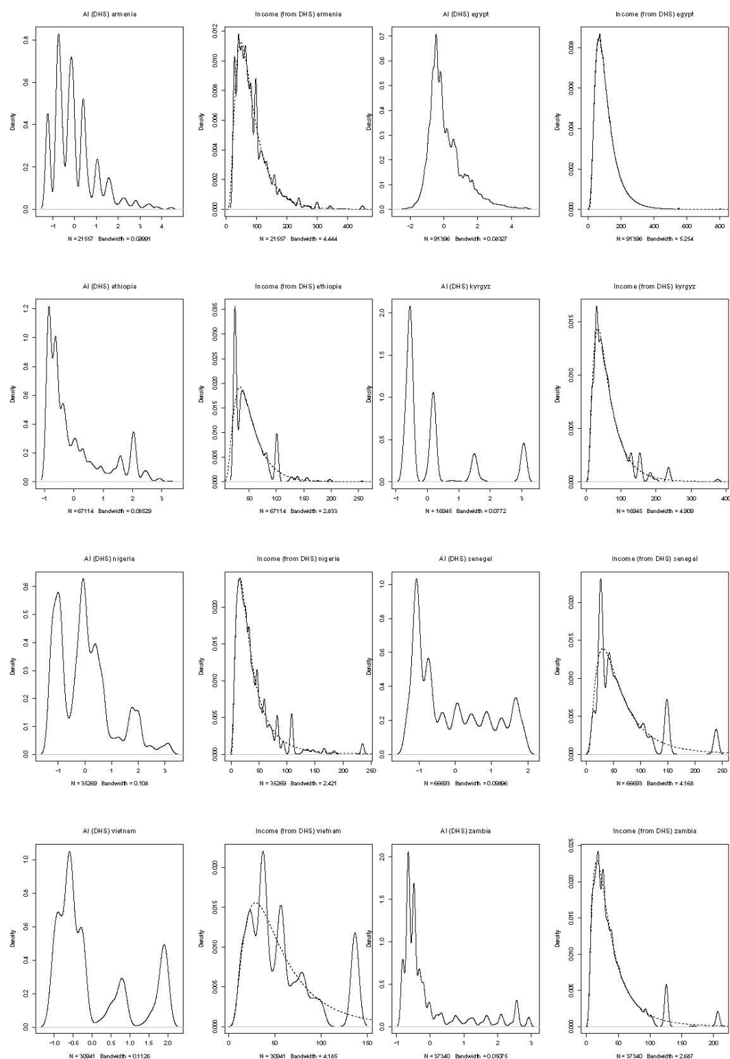
Figure A1: Distributions of the asst index and income
